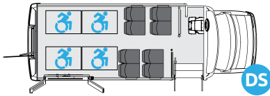
8 Passengers + 4 W/C
