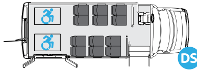
12 Passengers + 2 W/C
